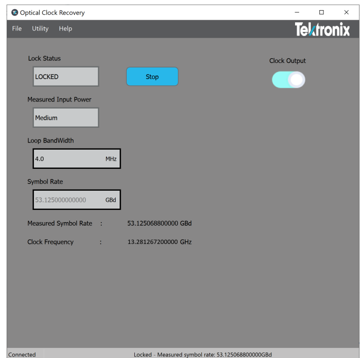
Figure 1: The user interface connected to a TCR801 Optical Clock Recovery and locked to a 53.125 Gb/s SSPRQ pattern
