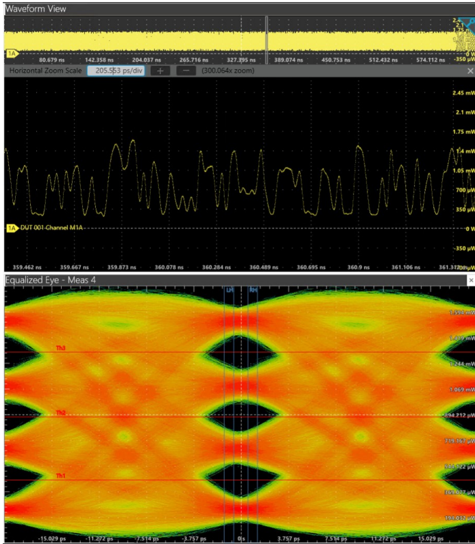
Figure 5: Example of a 53 Gb/s PRBS15 signal acquired on the Tektronix TSO820 Sampling Oscilloscope with TSO8C18 optical module, triggered by the TCR801 Optical Clock Recovery.
