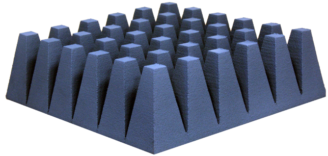
ETS-Lindgren's Model FS-200 Anechoic Absorber
