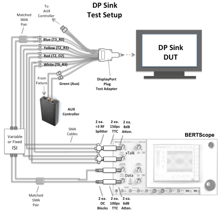
Test setup
