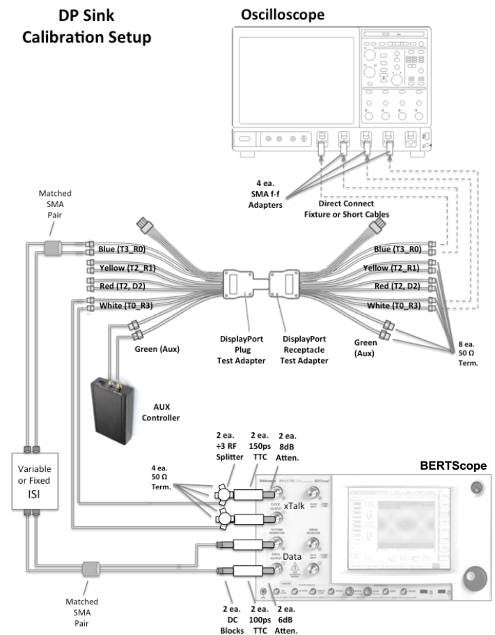
Calibration setup
